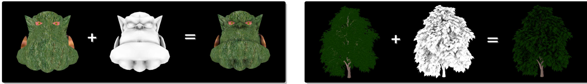
Figure 3: Composition of our viewpoint-based ambient occlusion and the textures of the Ogre (left) and tree models (right).
