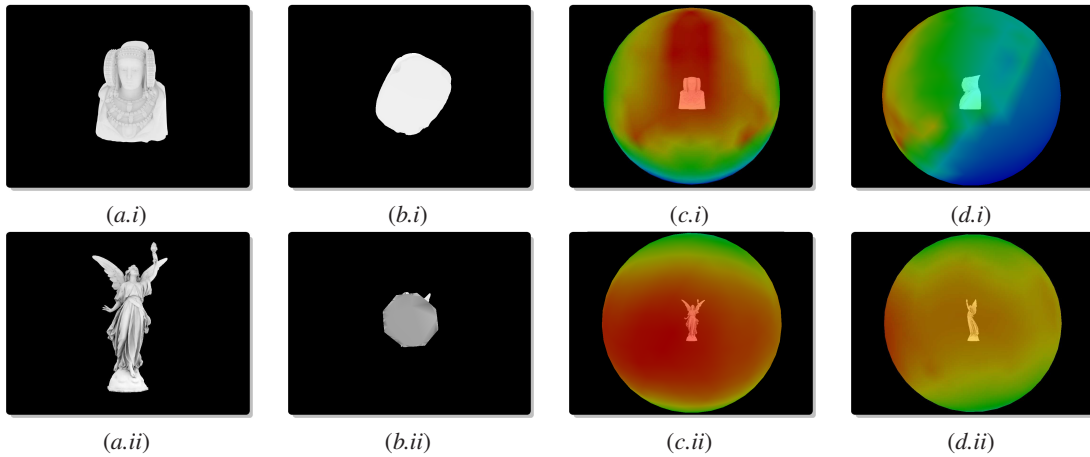
Figure 7: (a) The most and (b) least informative views of the Lady of Elche (i) and Lucy (ii) models. (c-d) Two different views of the PMI spheres.
