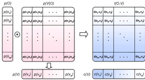
Figure 5: Probability distributions of channel O \rightarrow V , elements of matrix I(O, V) and color distribution c(V) assigned to the viewpoint sphere.
